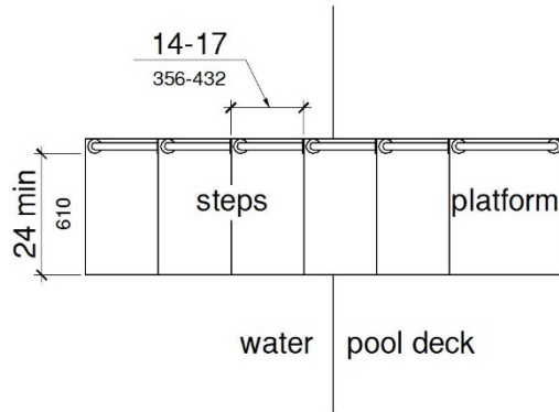
Figure 11B-1009.5.6 Size of Transfer Steps
