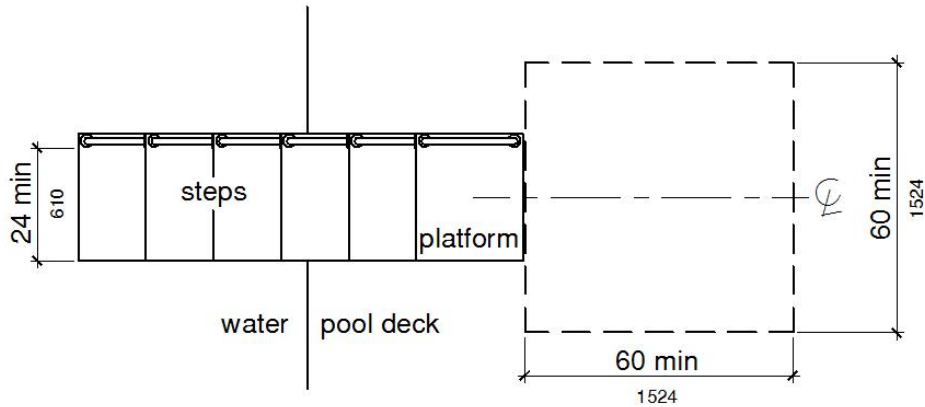
Figure 11B-1009.5.2 Clear Deck Space at Transfer Platform
