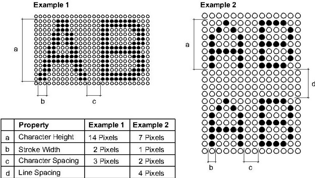
Figure 11B-703.8.5 Low Resolution VMS Characters
