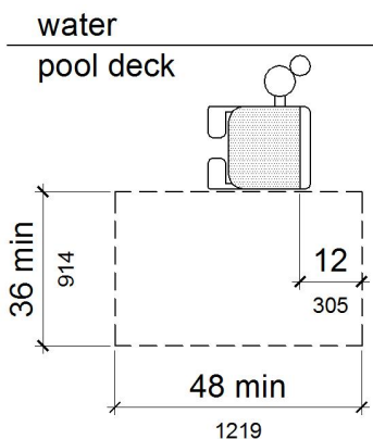
Figure 11B-1009.2.3
