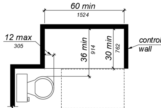
Figure 11B-809.10.6.1 Showers
