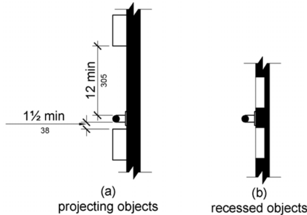
Figure 11B-609.3
