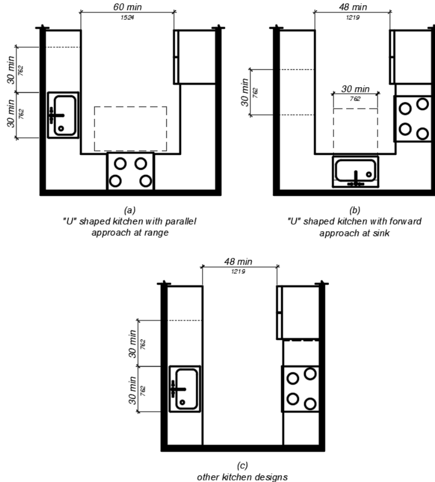
Figure 11B-809.2 Clear Width at Kitchens
