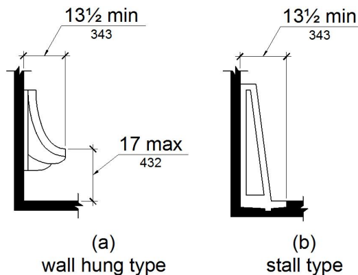
Figure 11B-605.2
