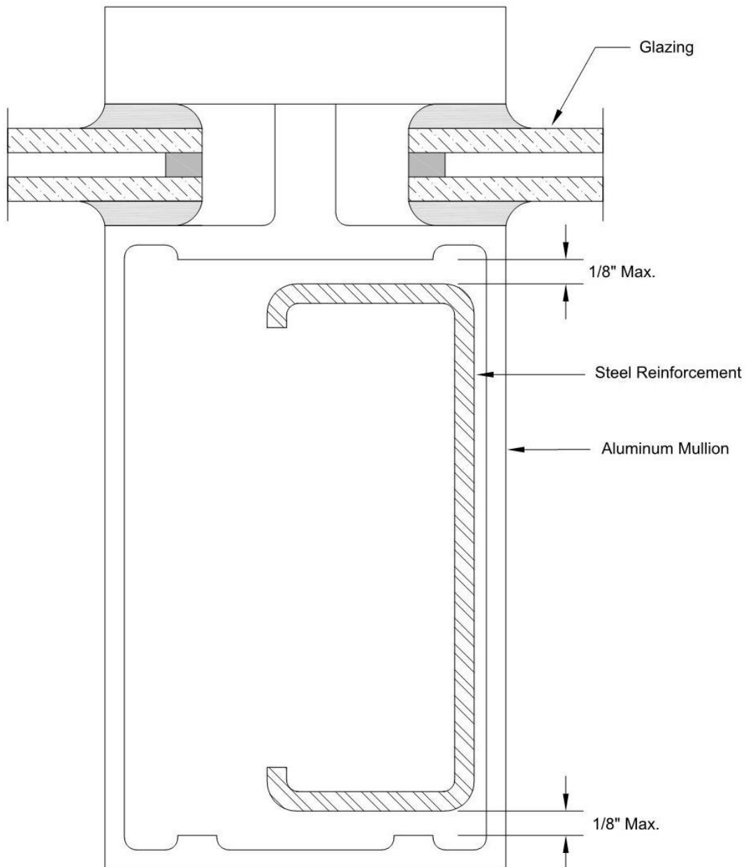
Figure 2.5: Steel Reinforced Mullion
